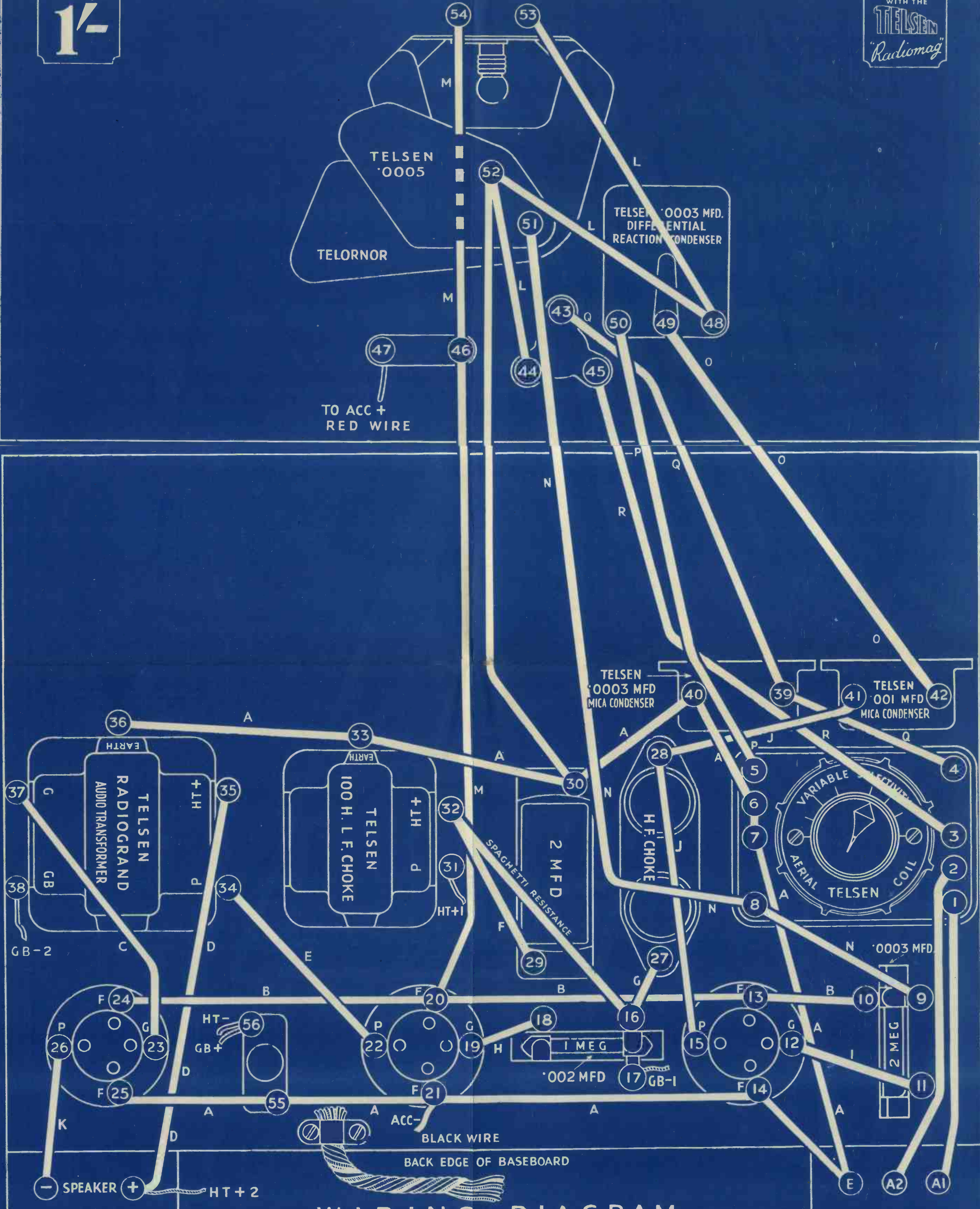
WIRING DIAGRAM
